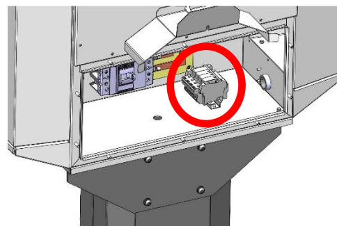
Figure 30 - Surge Protective Device that contains replaceable surge modules
