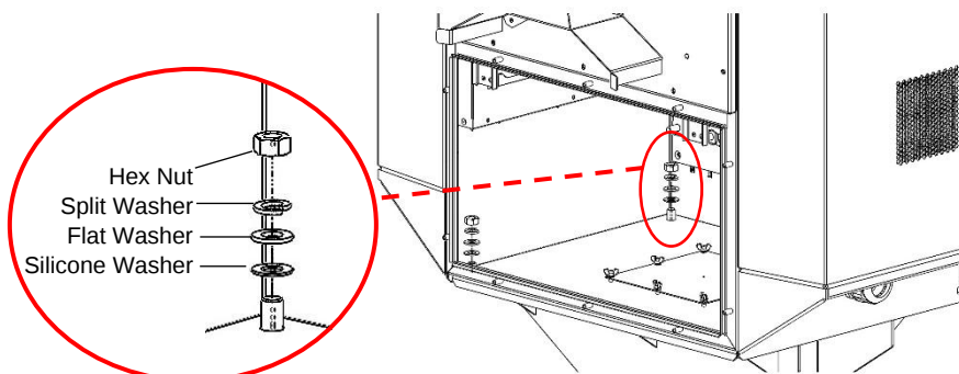
Figure 12 - Securing charger to pedestal with hardware provided
