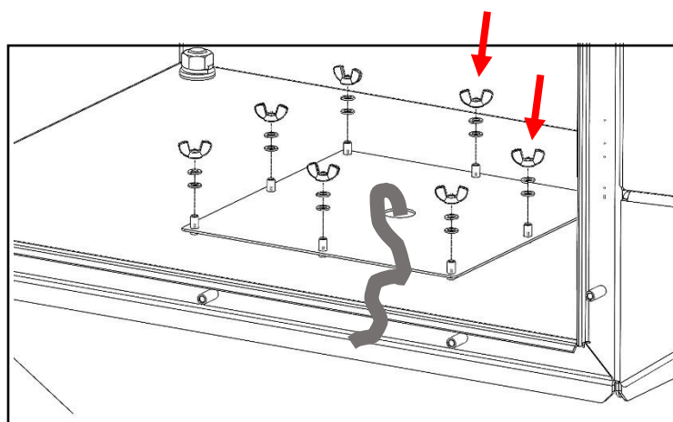
Figure 15 - Placement of Removable Plate inside bottom of charger (optional Cable Gland not shown)
