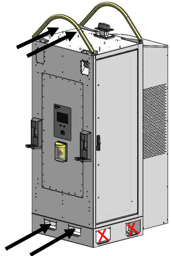
Figure 15 – Forklift forks may be inserted into either the two open front panels or 2 lifting straps connected to eye bolts on top of charger
