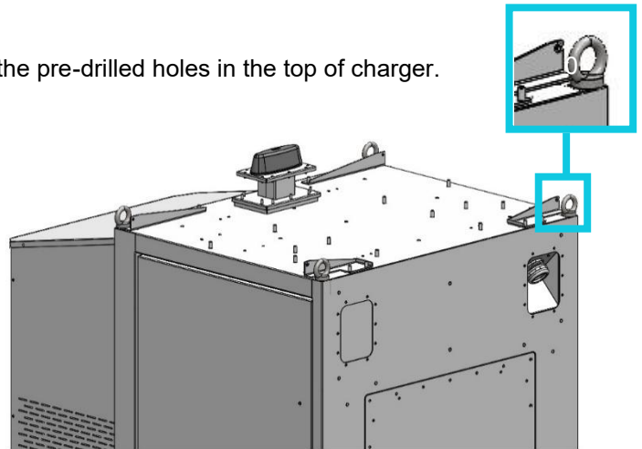
Figure 18 – Installing eye bolts
