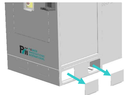
Figure 13 - Removing left and right access panels to access 4 hex bolts and washers securing charger to pallet
