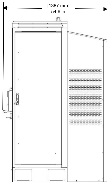
Figure 4.1 – Dimensions of 60 kW Bi-directional charger WITHOUT cable management
